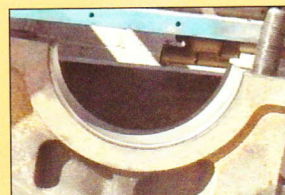
Crankshaft Main Bearings looked like new, there were no traces of wear. They maintained their original coating. Usually after 17,000 work-hours they are chewed up. In this engine we used Polytron, there was almost no wear at all after 30,000 work-hours.
