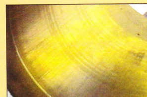
Cylinder liner from a 16,000 work-hours old engine (without Polytron MTC ) scuffed and scored.
