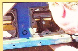
We micro-measured the crankshaft and found it to be in great condition. Totally round, no traces of wear. It didn't need any machining.
